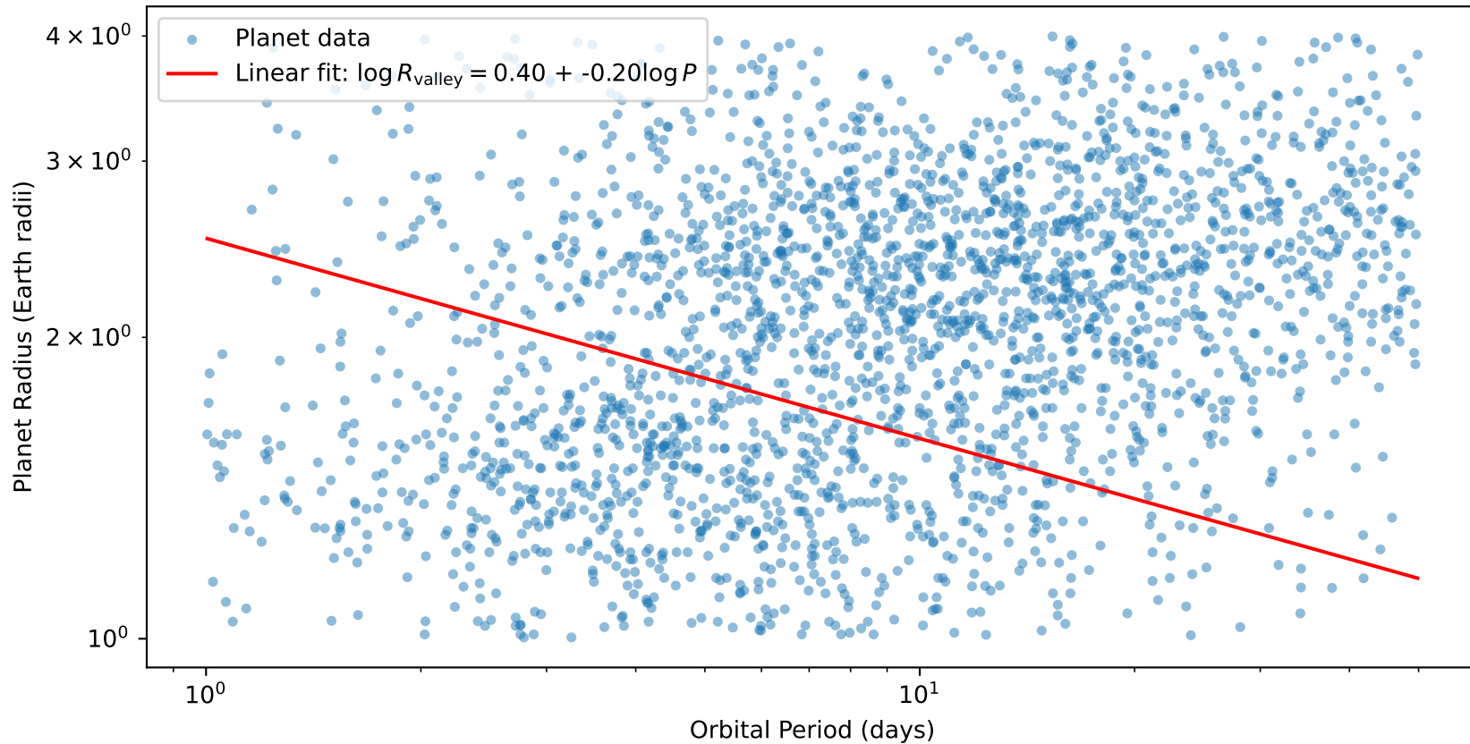
Exoplanet Radius vs. Orbital Period
